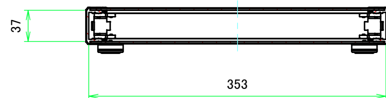
B-B (1:4.5)
