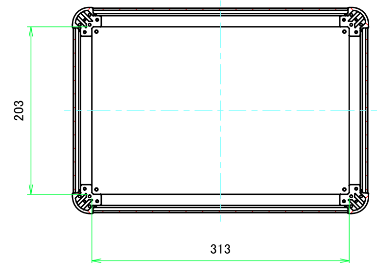
C-C (1:4.5)
